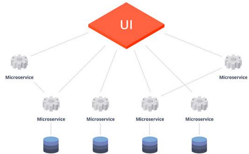
Microservice Architecture
